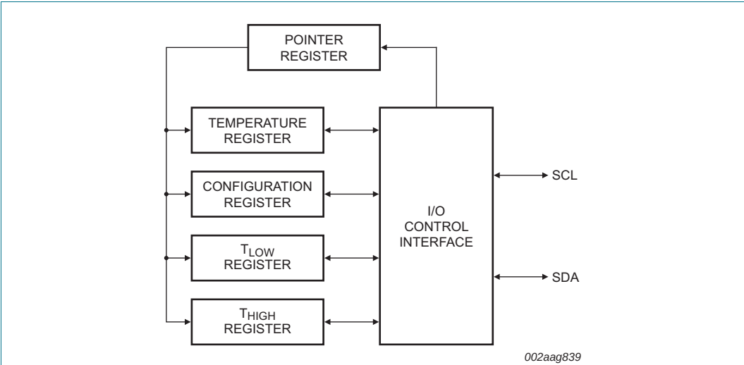
Fig 4. Internal register structure
