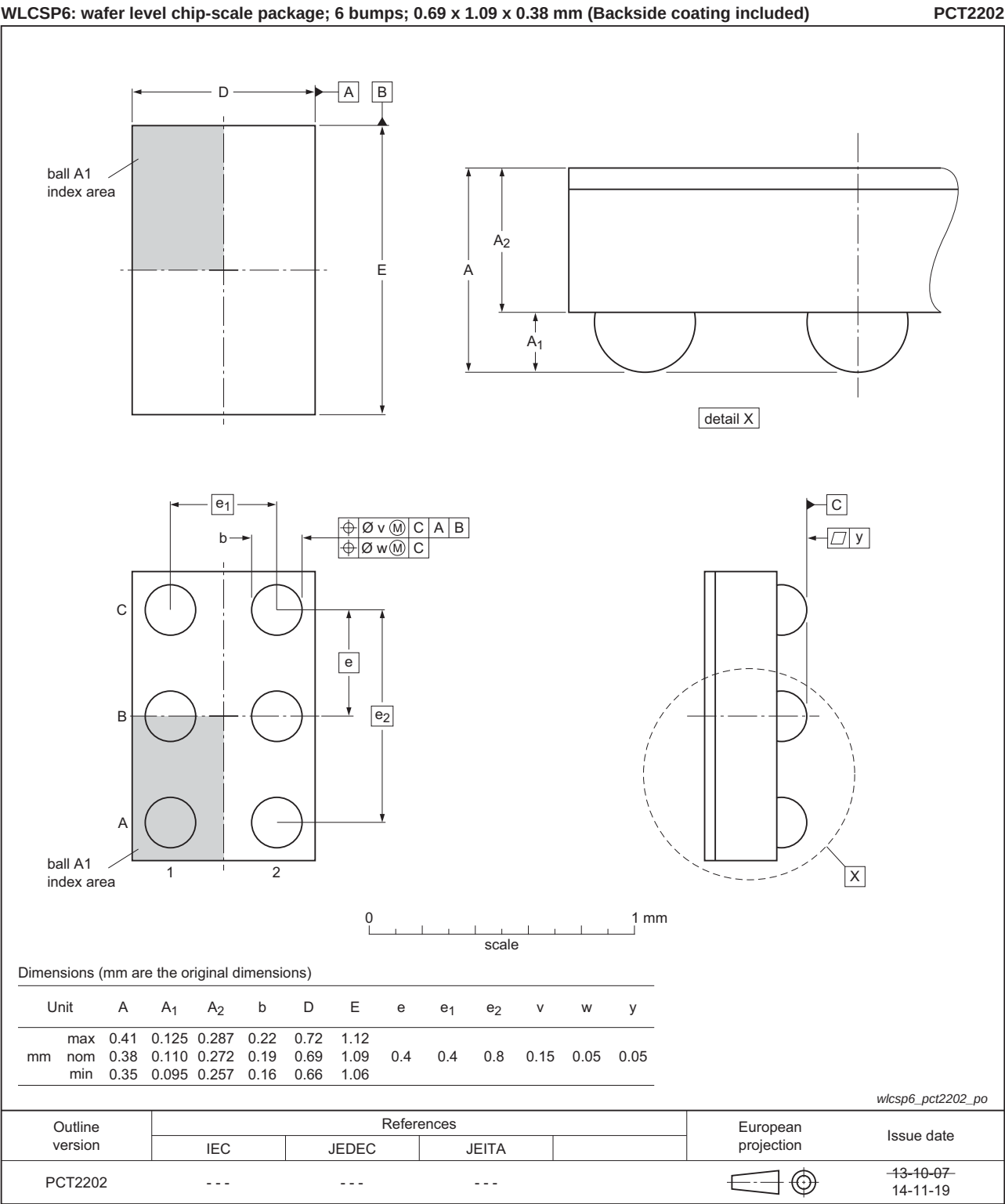
Fig 18. Package outline PCT2202UK (WLCSP6)
