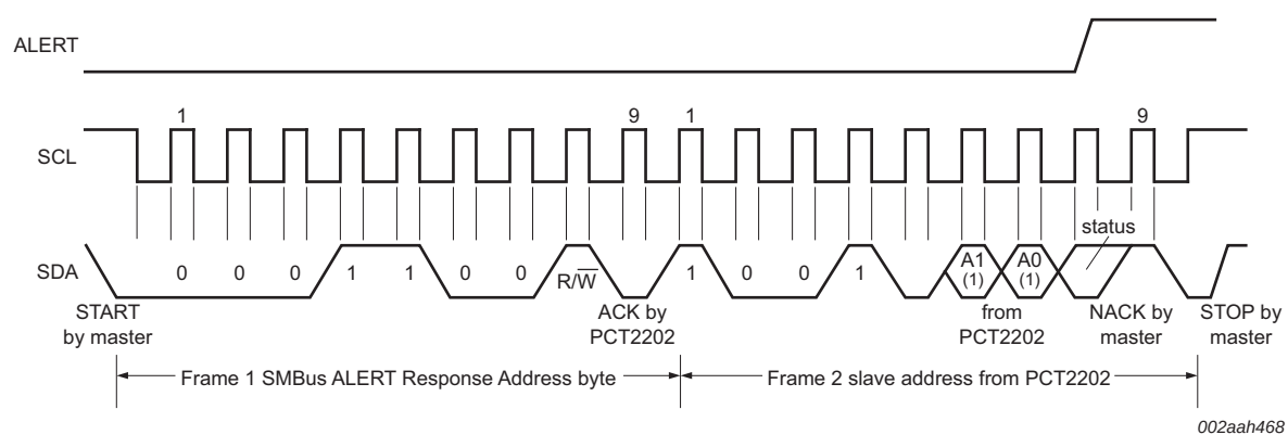
Fig 17. Timing diagram for SMBus ALERT
